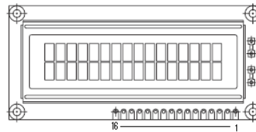
Gambar 7. LCD
