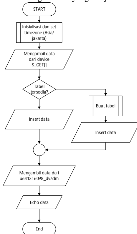
Gambar 13. Flowchart upload.php
